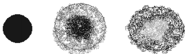
Fig. 3—The first picture represents zero error in the visual system and thus an image sharply in focus at the retina. The next 2 represent blur circles created when spherical aberration is present such that all incoming rays of light do not focus at the same location on the retina. The darker centre and lighter surround represent positive spherical aberration (peripheral rays focus in front of the central point), and the final picture represents negative spherical aberration (central rays come to a focus in front of peripheral).
