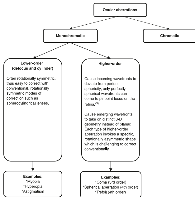
Fig. 1—Simplified classification of ocular aberration. Ocular aberrations are imperfections in the ocular media, changes in refractive index, and misalignments of the ocular media, which prevent rays of light that emerge from an object from coming to a sharp focus together at the same point on the retina, regardless of their direction of travel or point of entry into the pupil.
